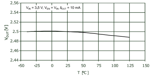
Figure 5: V_{OUT} accuracy
