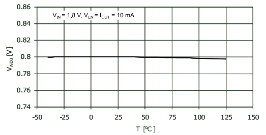
Figure 4: V_{ADJ} accuracy
