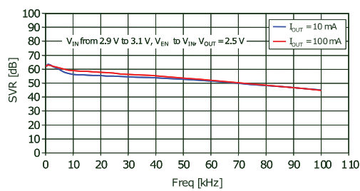
Figure 20: Supply voltage rejection vs. frequency ( V_{OUT} = 2.5 V)
