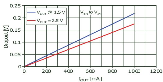
Figure 8: Dropout voltage vs. output current
