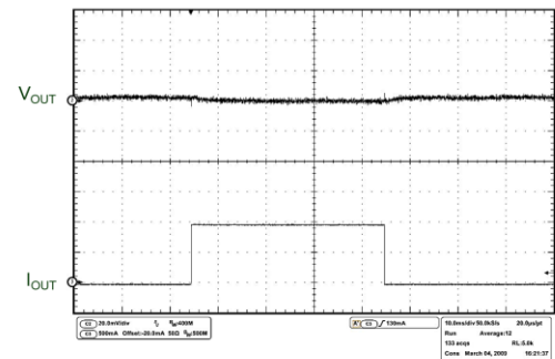
Figure 23: Load Transient ( V_{OUT} = 0.8 V, I_{OUT} = from 10 mA to 1 A)
