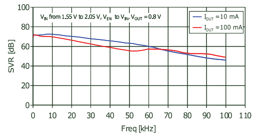
Figure 19: Supply voltage rejection vs. frequency ( V_{OUT} = 0.8 V)
