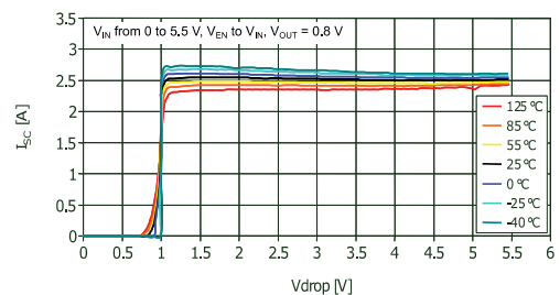
Figure 9: Short-circuit current vs. drop voltage
