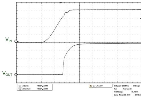
Figure 28: Start-up transient
