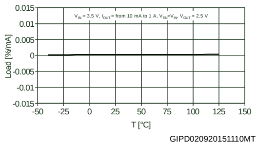
Figure 14: Load regulation
