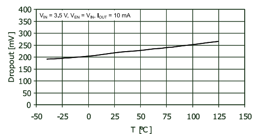
Figure 7: Dropout voltage vs. temperature ( V_{OUT} = 1.5\text{ V} )
