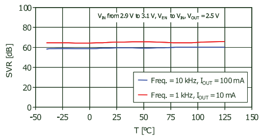
Figure 18: Supply voltage rejection vs. temperature ( V_{OUT} = 2.5 V)
