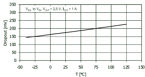
Figure 6: Dropout voltage vs. temperature ( V_{OUT} = 2.5\text{ V} )
