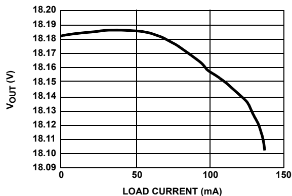
FIGURE 9. LOAD REGULATION ( V_{IN} = 3.6V )
