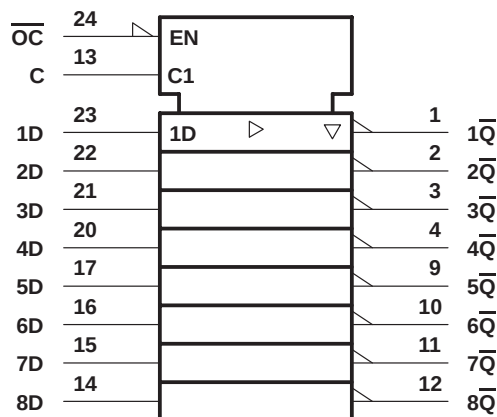
logic symbol †
