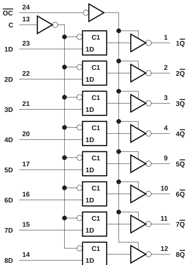
logic diagram (positive logic)
