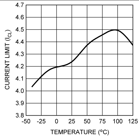
Figure 2. Current Limit vs Temperature
