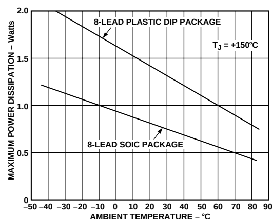
Figure 2. AD8180 Maximum Power Dissipation vs. Temperature
