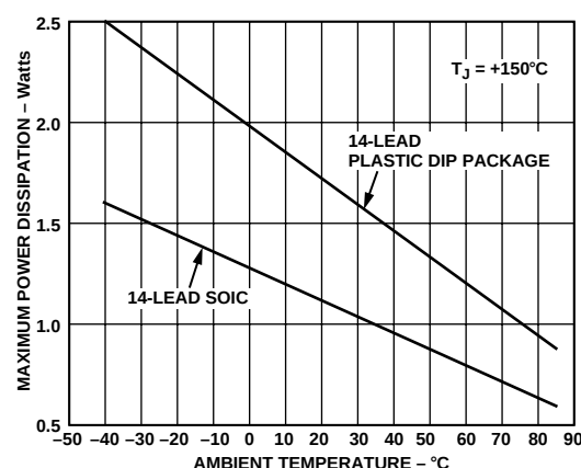
Figure 3. AD8182 Maximum Power Dissipation vs. Temperature
