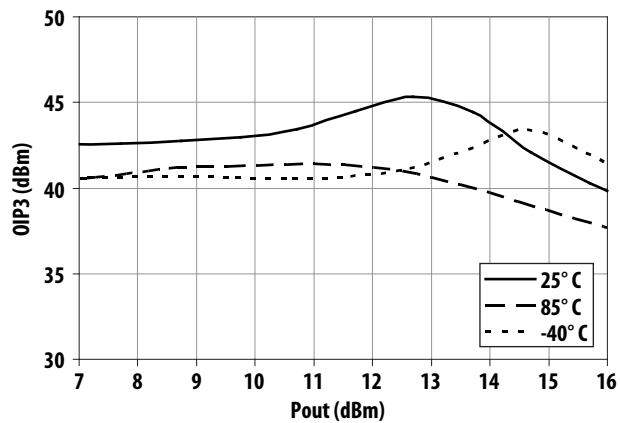
Figure 24. Over Temperature OIP3 vs Pout at 2600 MHz
