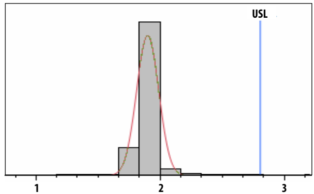
Figure 5. NF at 1900 MHz, Vdd = 5 V, Nominal = 1.9 dB, USL = 2.8 dB
