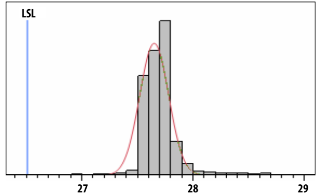
Figure 3. OP1dB at 1900 MHz, Vdd = 5 V, LSL = 26.3 dBm, Nominal = 27.6 dBm
