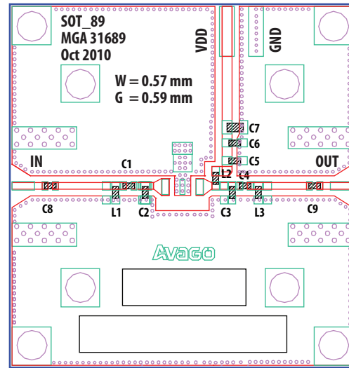
Figure 28. Demo board
