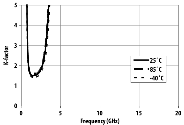
Figure 16. Over Temperature K-factor vs Frequency
