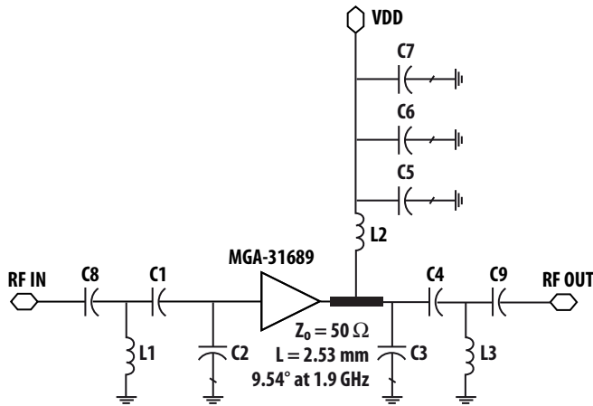
Figure 27. Circuit diagram
