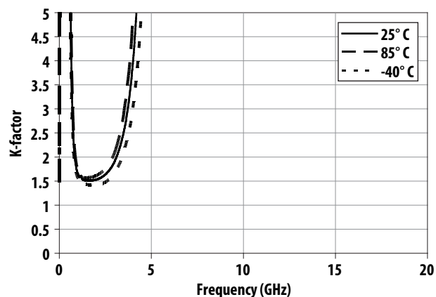
Figure 26. Over Temperature K-factor vs Frequency
