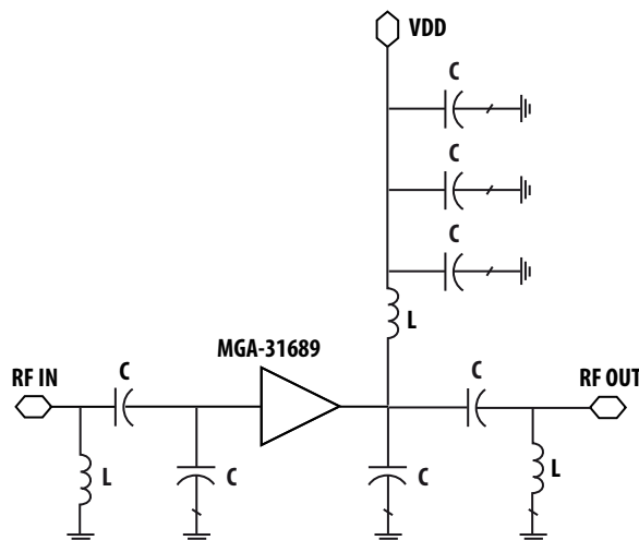
Figure 1. Simplified Schematic diagram
