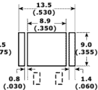
Recommended Heat Sink Solder Mask Opening
