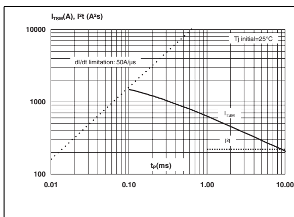
Figure 7. Non repetitive surge peak on-state current (sinusoidal pulse width t_p < 10 ms ) and value of I^2t
