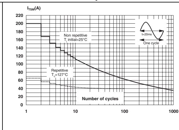
Figure 6. Surge peak on-state current vs number of cycles
