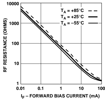
Figure 2. RF Resistance vs. Forward Bias Current.
