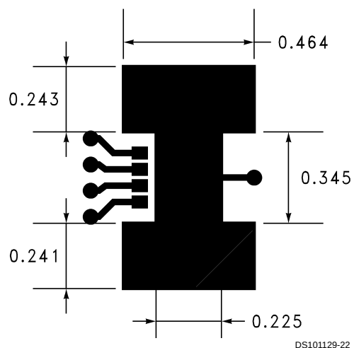
FIGURE 8. SCENARIO C, \theta_{JA} = 92^{\circ}\text{C/W}
