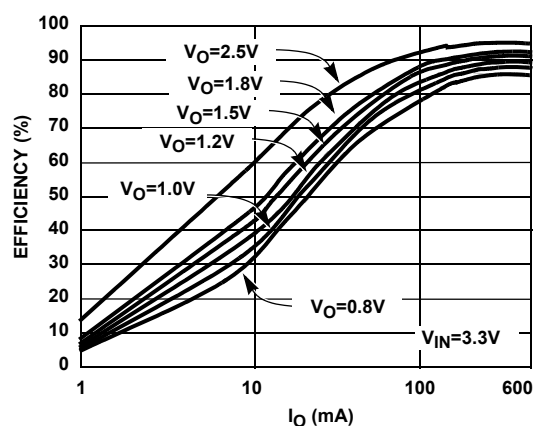
FIGURE 4. EFFICIENCY vs I_O (PWM MODE)
