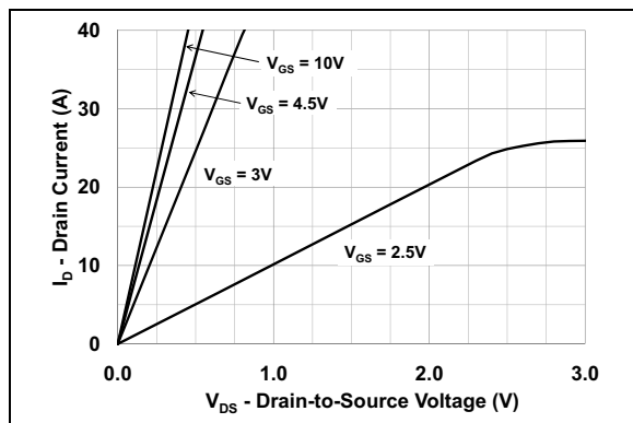
FIGURE 2-1: Typical Output Characteristics.
