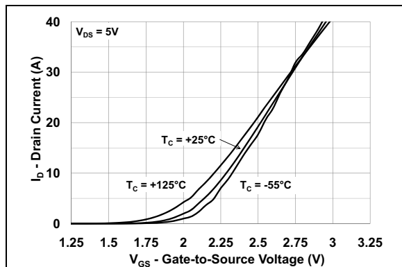
FIGURE 2-2: Typical Transfer Characteristics.
