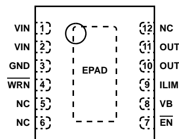
ISL9212 (12 LD 4x3 TDFN) TOP VIEW
