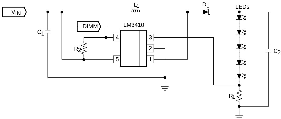
Figure 21. LM3410X (1.6 MHz) 5 × 3.3-V LED String Application Diagram
