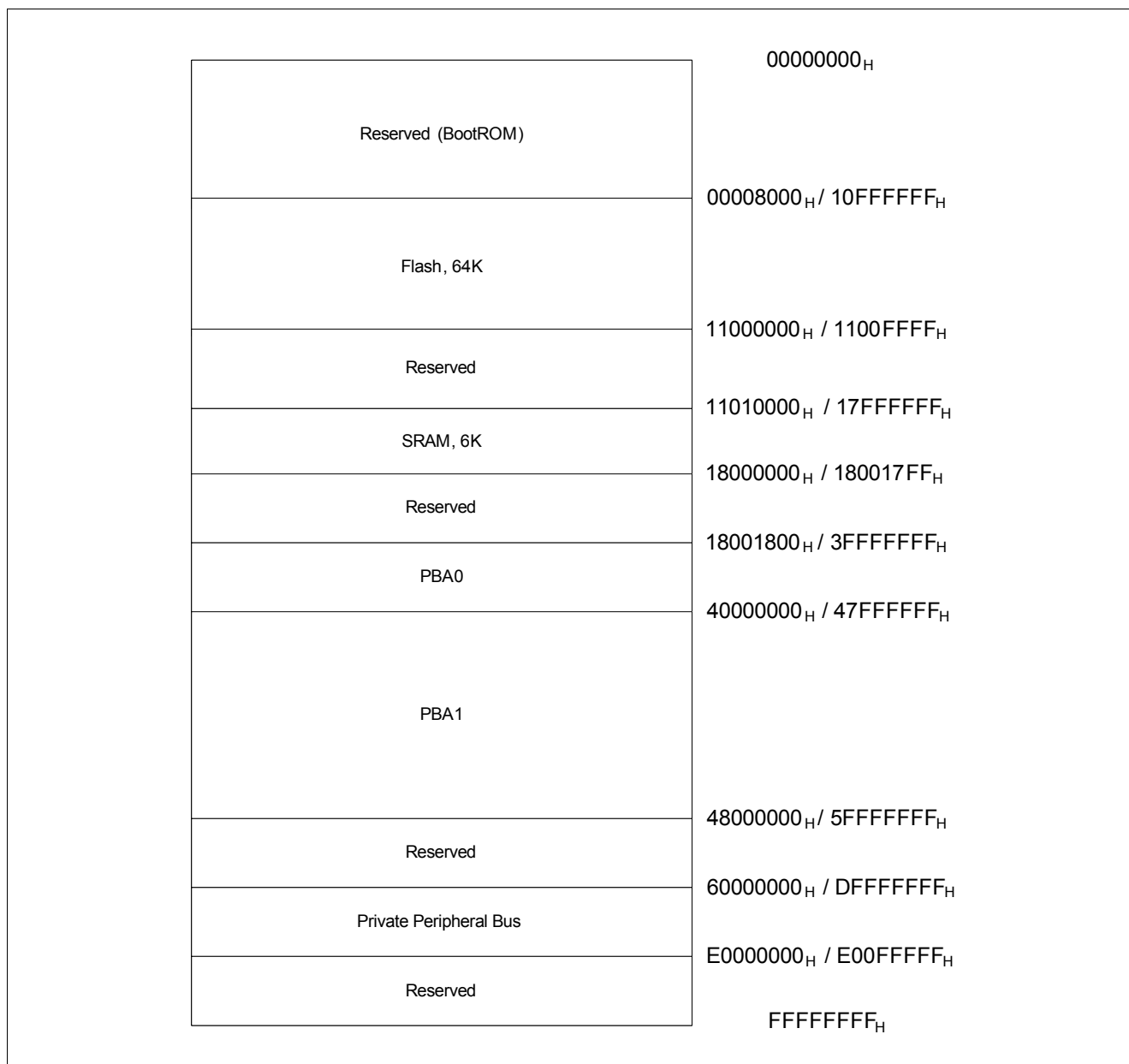
Figure 14 TLE9877QXA20 Memory Map
