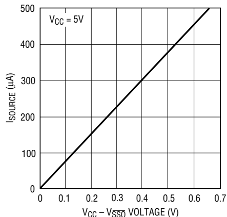
LTC1296 \overline{SSO} Source Current vs V_{CC} - V_{SS0}
