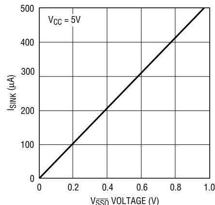
LTC1296 \overline{SSO} Sink Current vs V_{SS0}
