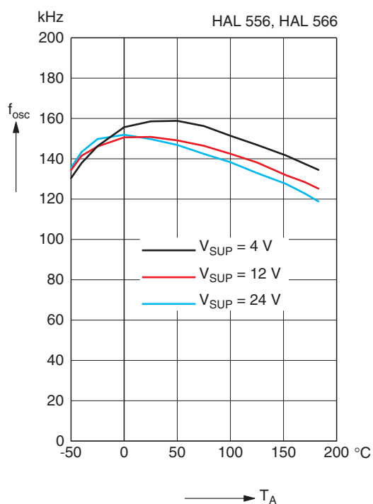
Fig. 4-6: Typ. internal chopper frequency versus ambient temperature
