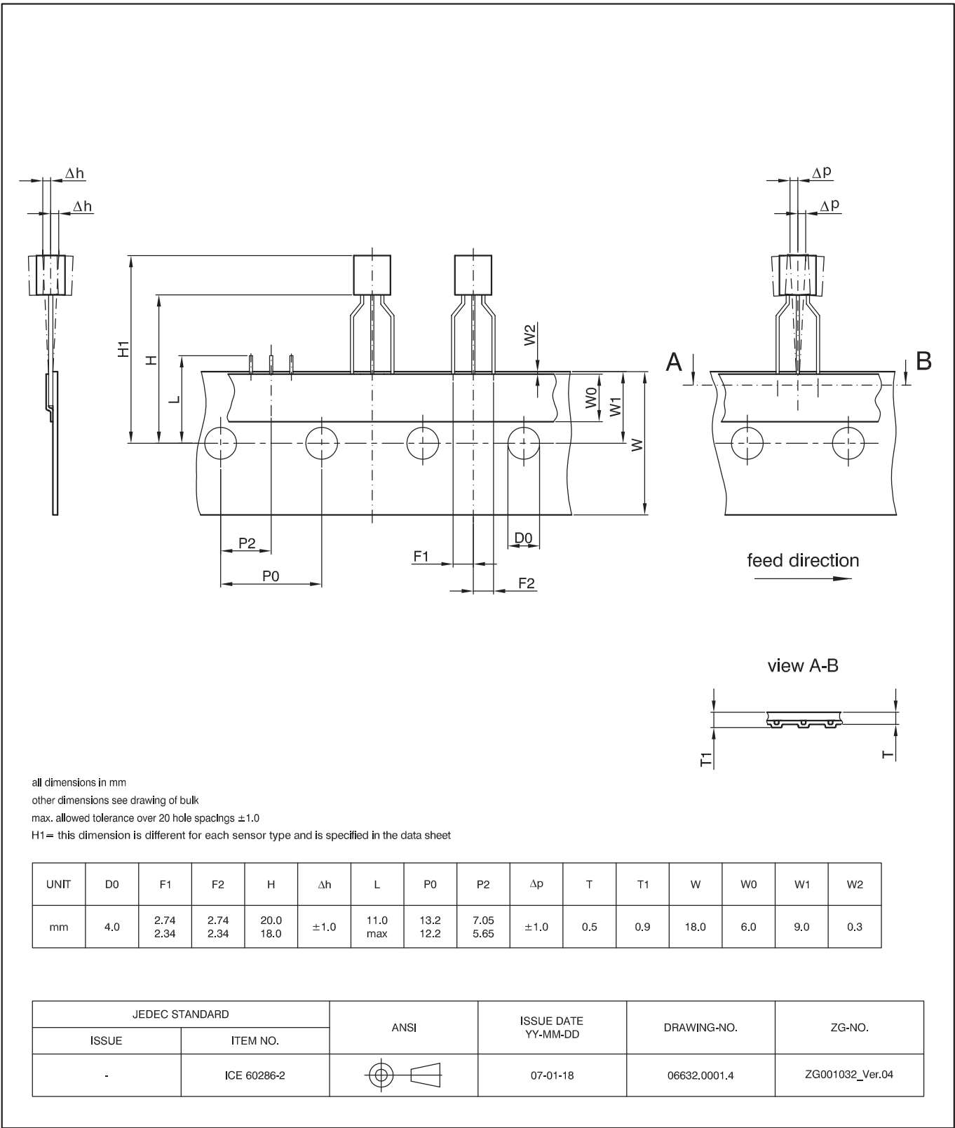
Fig. 4-2: TO92UA-1: Dimensions ammopack inline, spread
