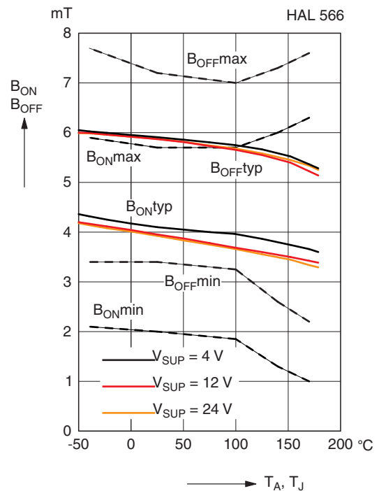
Fig. 5-8: Magnetic switching points versus temperature
