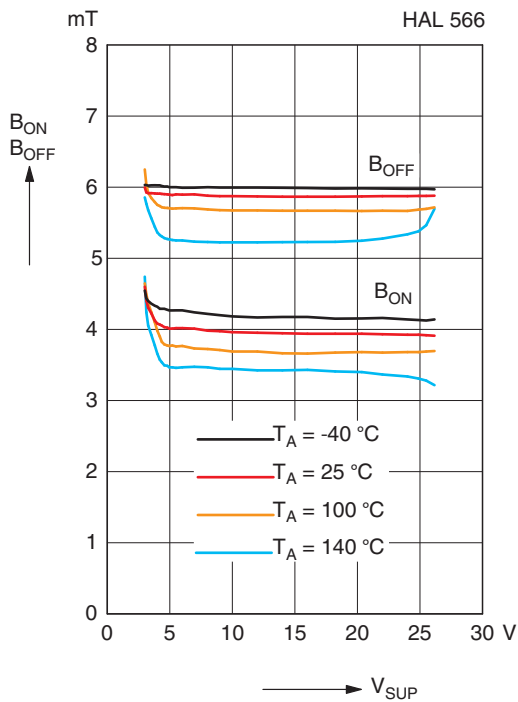
Fig. 5-6: Typ. magnetic switching points versus supply voltage
