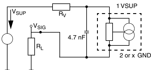
Fig. 6–2: Application circuit 2
