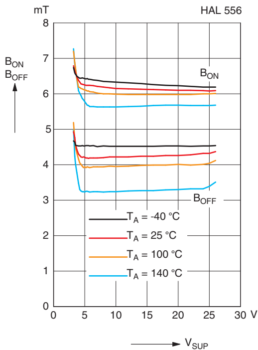
Fig. 5-2: Typ. magnetic switching points versus supply voltage
