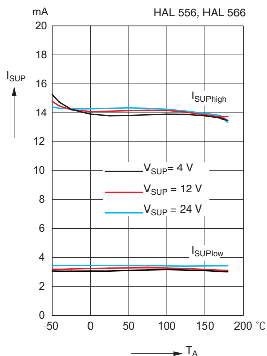
Fig. 4-5: Typical supply current versus ambient temperature
