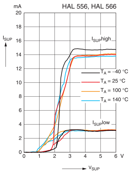
Fig. 4-4: Typical supply current versus supply voltage
