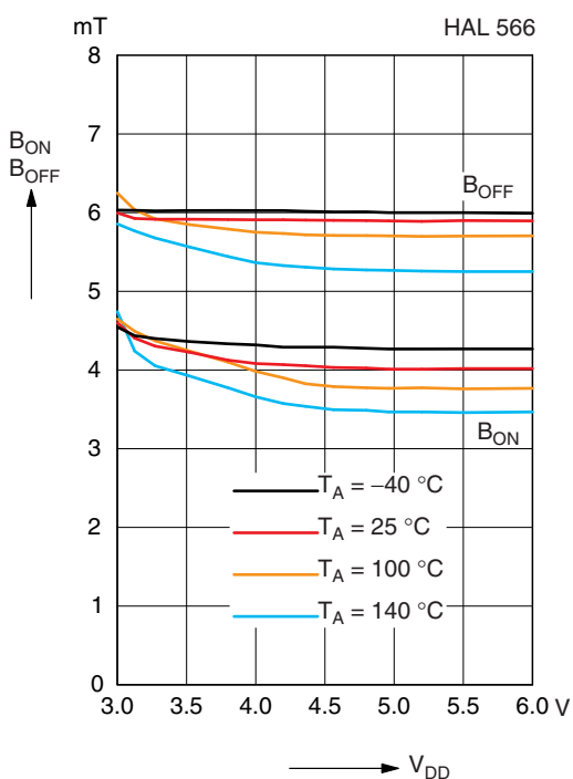
Fig. 5-7: Typ. magnetic switching points versus supply voltage
