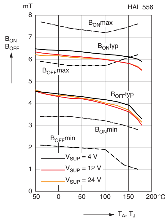
Fig. 5-4: Magnetic switching points versus temperature
