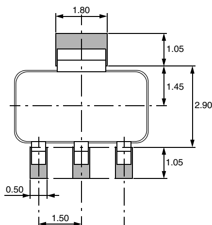
Fig. 4-2: Recommended pad size SOT89B-1 Dimensions in mm
