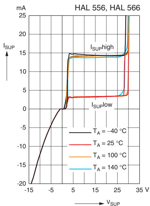
Fig. 4-3: Typical supply current versus supply voltage
