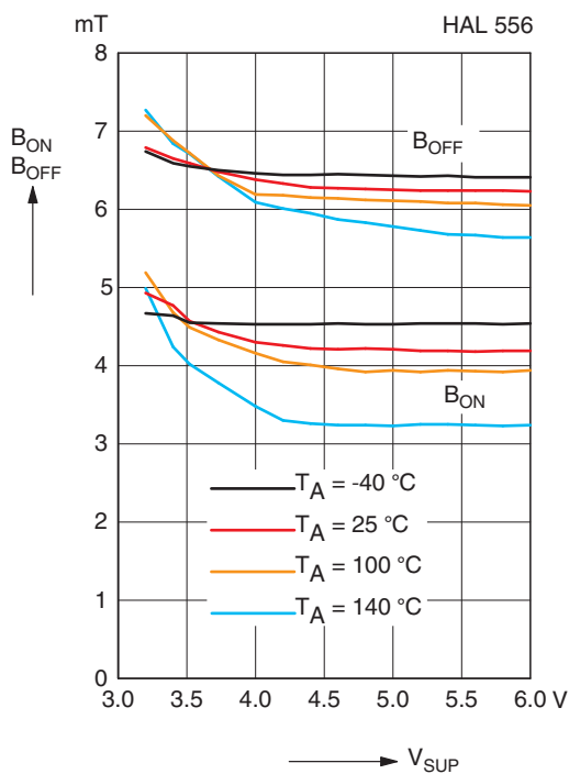
Fig. 5-3: Typ. magnetic switching points versus supply voltage
