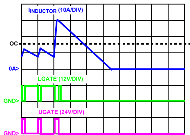
FIGURE 5. OCP TIMING (ISL6341A, ISL6341C)
