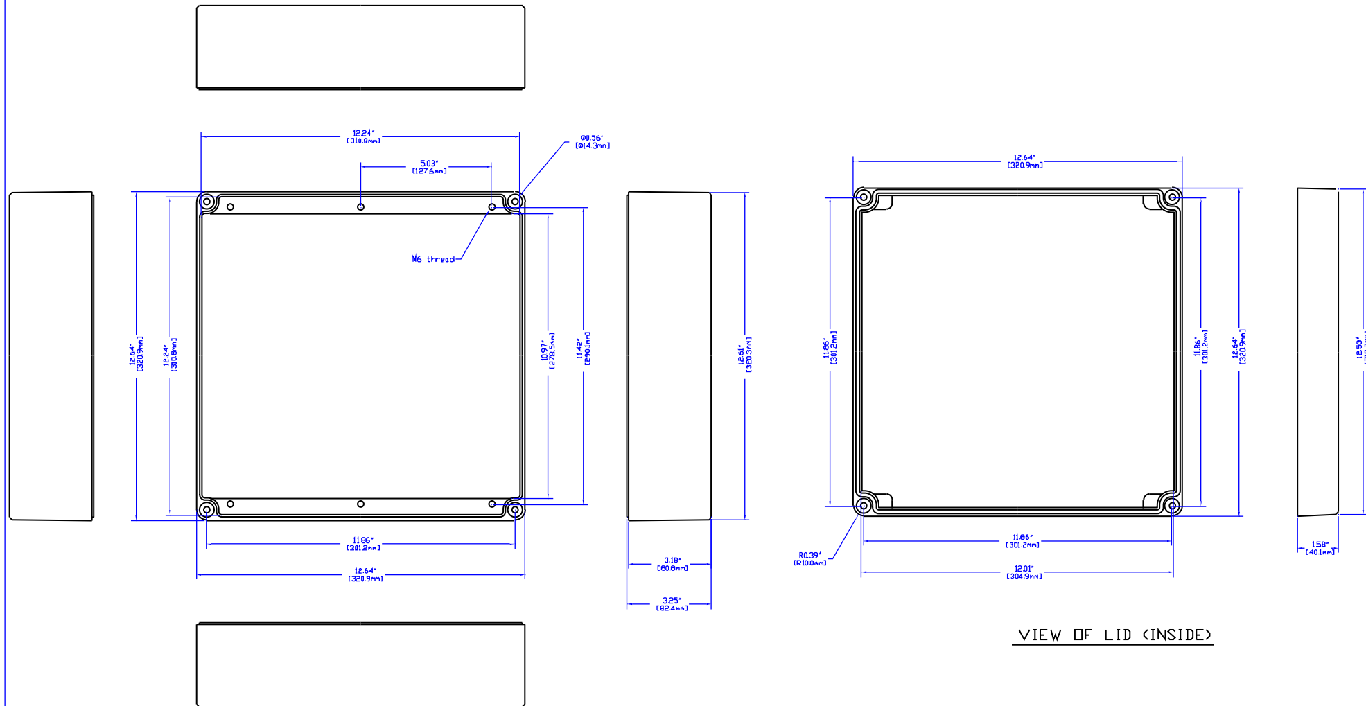
VIEW OF BOX (LID REMOVED)
