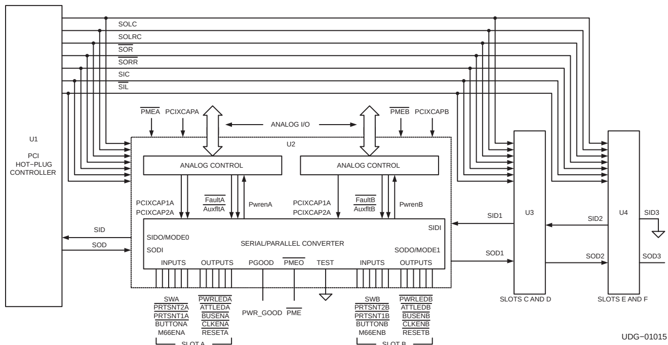
Figure 1. Hot-Plug System Block Diagram
