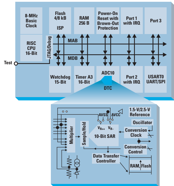
MSP430F169—The industry's first complete MCU-based SCoC.
