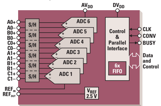
ADS8364 Block Diagram
