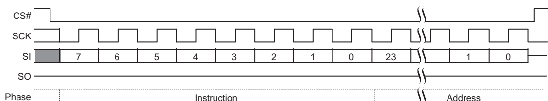
Figure 9.30 Erase Security Registers Command Sequence
