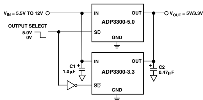
Figure 22. Crossover Switch
