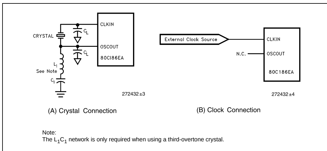
Figure 2. Clock Configurations
