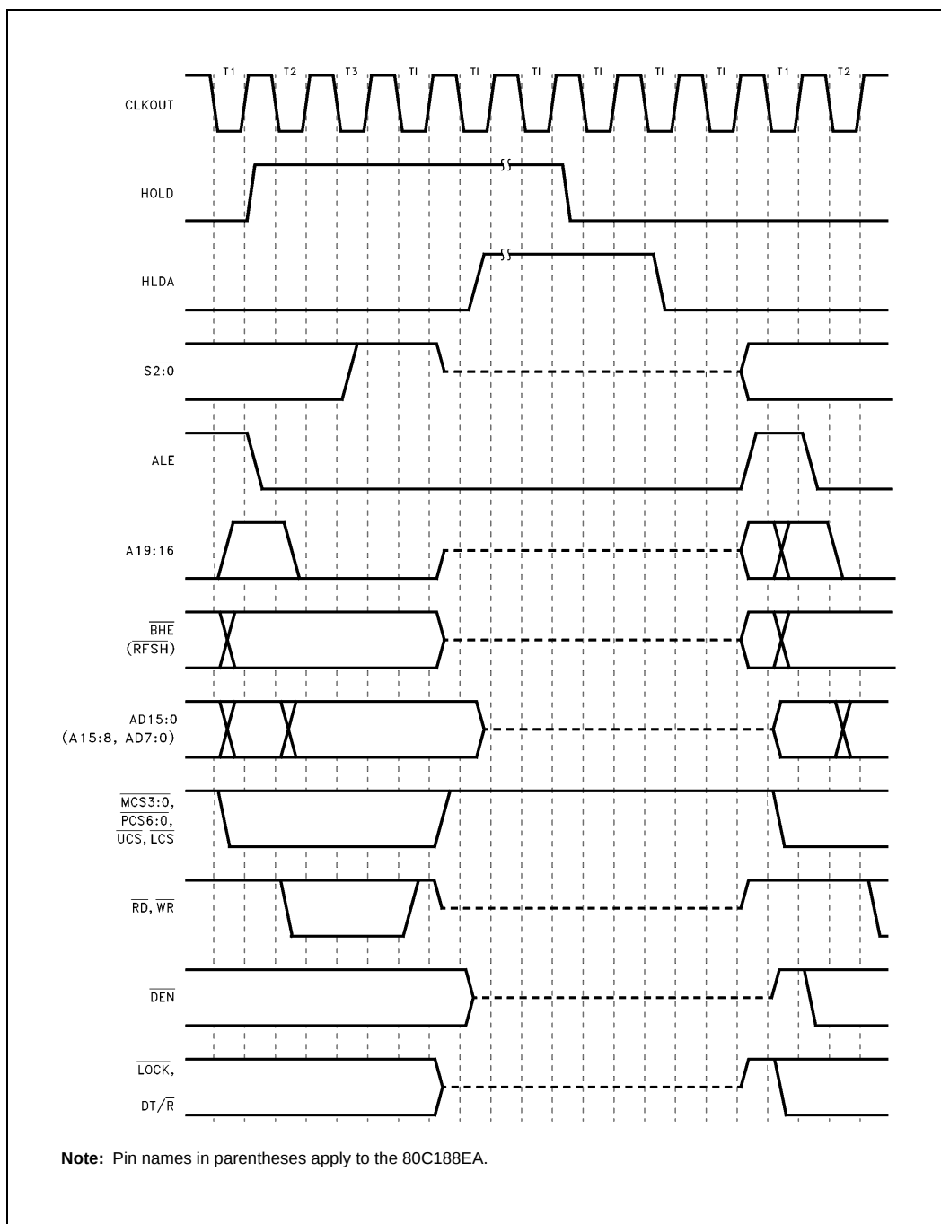
Figure 17. HOLD/HLDA Waveform
