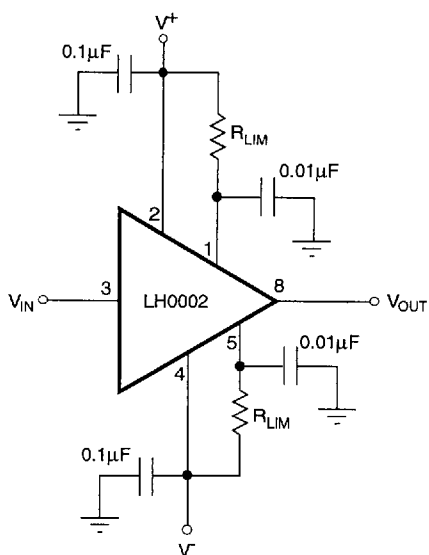
FIGURE 5. LH0002 Using Resistor Current Limiting
