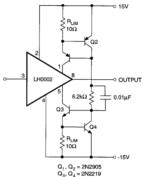
FIGURE 6. Current Limit Using Current Source
