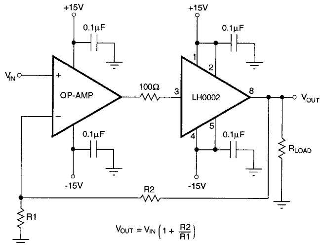
FIGURE 3. Non-Inverting Buffer Amplifier with Gain
