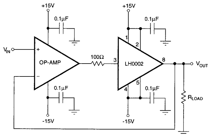
FIGURE 4. Non-Inverting Buffer Amplifier
