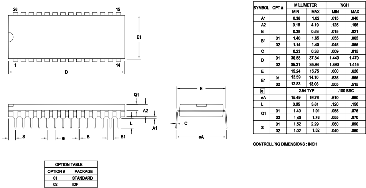
Figure 45 displays the 28-pin Plastic Dual Inline Package (PDIP) available for the Z8 Encore! XP F082A Series devices.
