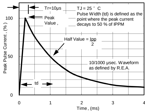
Fig. 4 - Pulse Waveform
