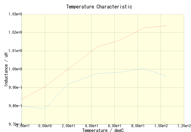
VLF403215MT-1R0N-CA(DC = 0A) VLF403215MT-1R0N-CA(DC = 1.505A)
