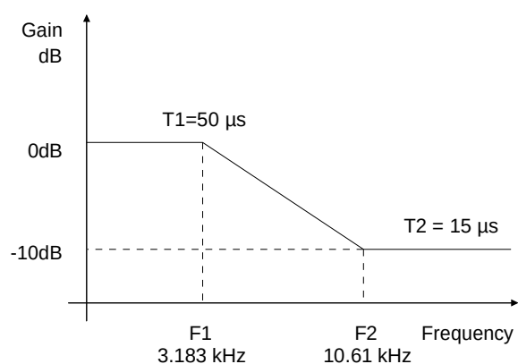
Figure 6. De-Emphasis Curve
