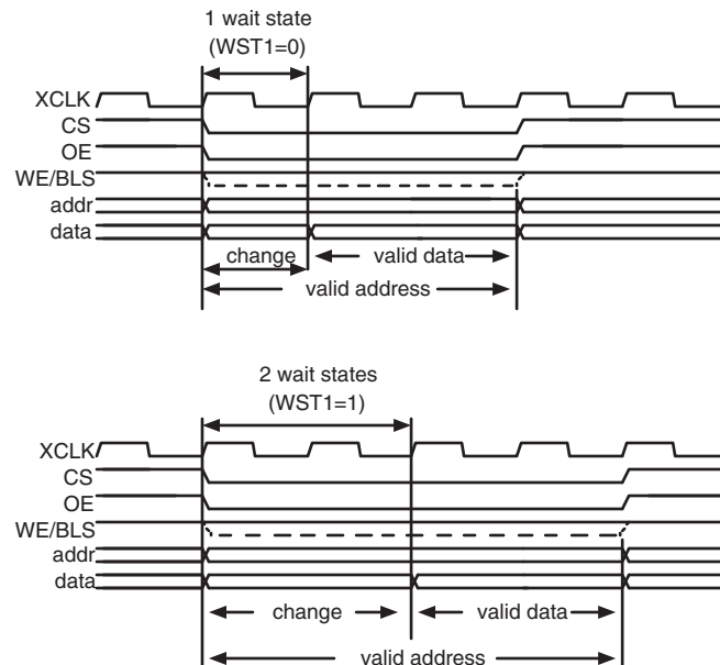
Fig 9. External memory read access (WST1 = 0 and WST1 = 1 examples)
