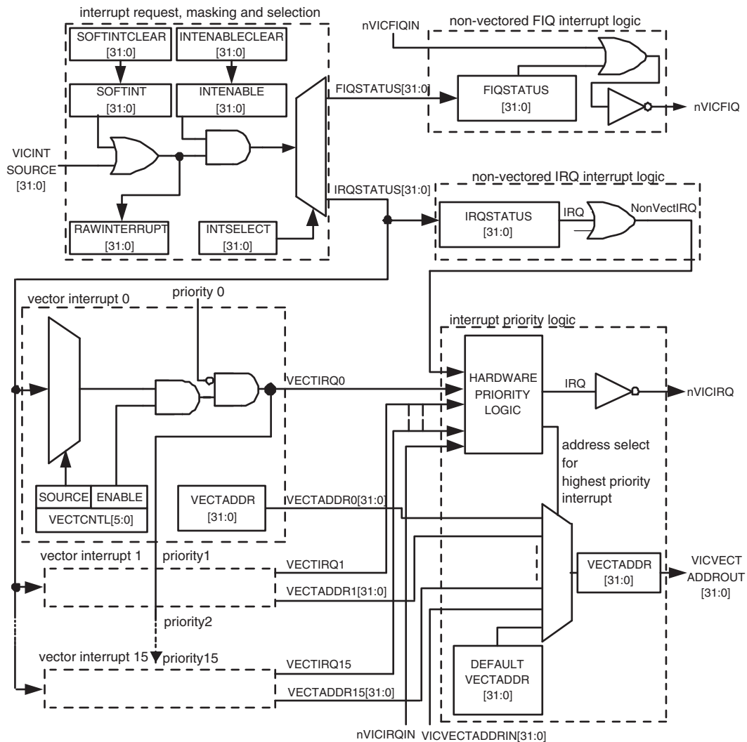
Fig 18. Block diagram of the Vectored Interrupt Controller (VIC)
