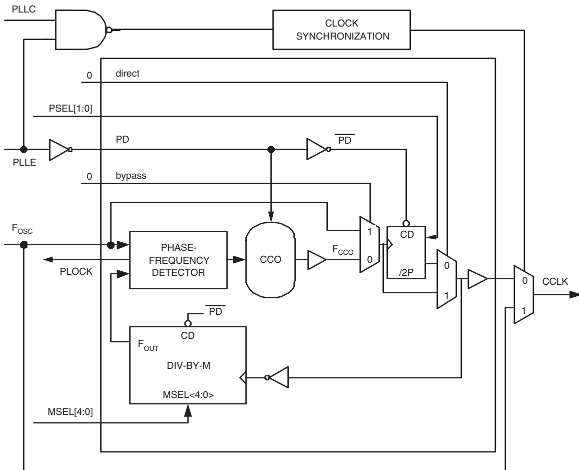
Fig 15. PLL block diagram
