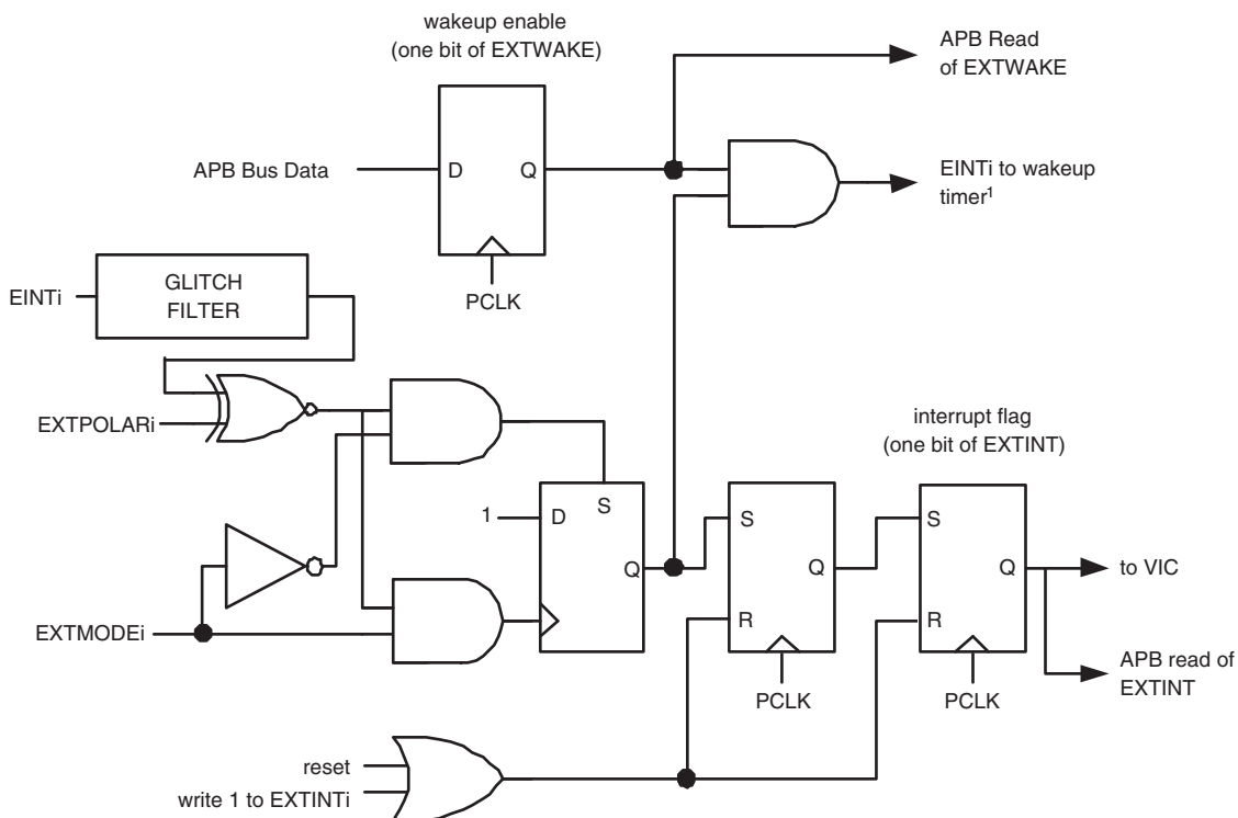
Fig 14. External interrupt logic
