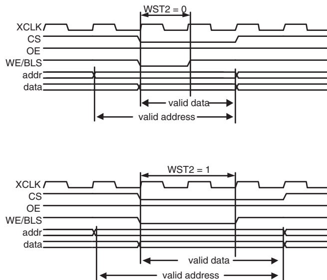
Fig 10. External memory write access (WST2 = 0 and WST2 = 1 examples)
