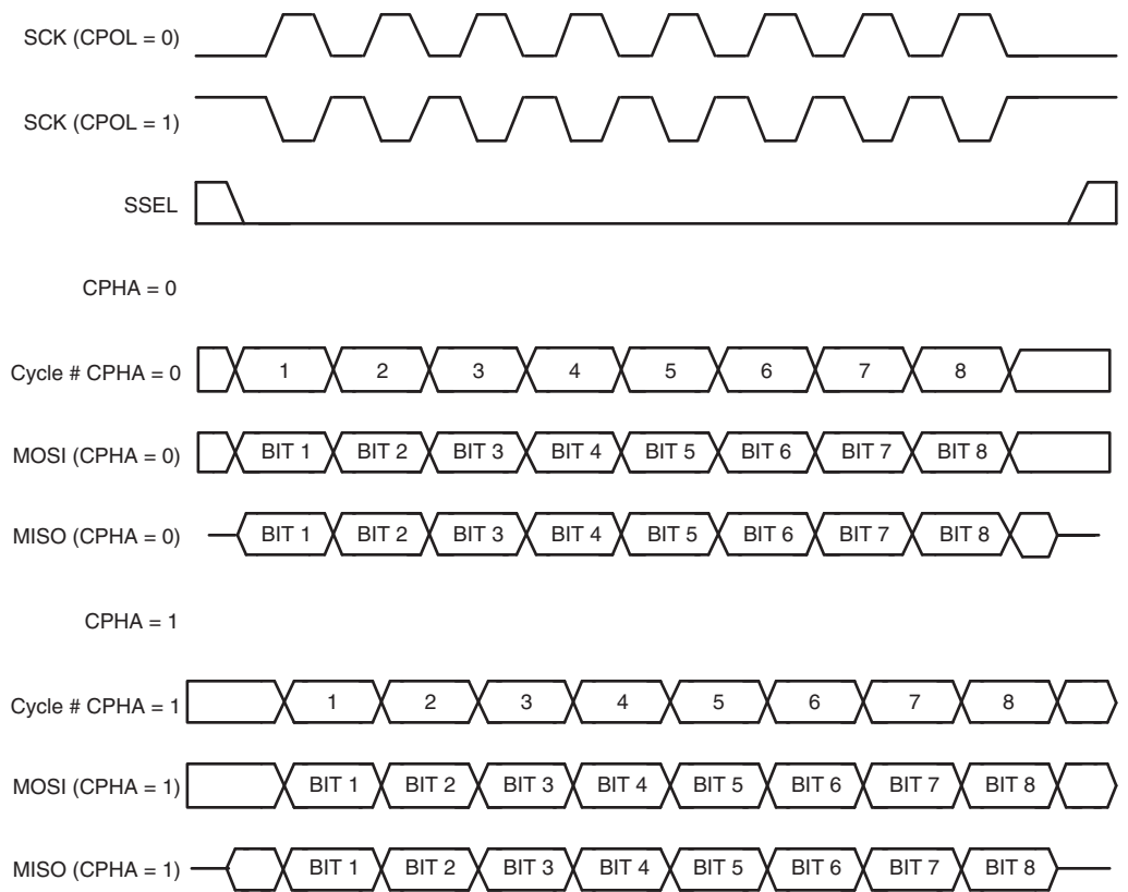
Fig 44. SPI data transfer format (CPHA = 0 and CPHA = 1)
