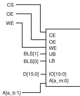
b. 16 bit wide memory bank interfaced to 16 bit memory chips (RBLE = 1)
