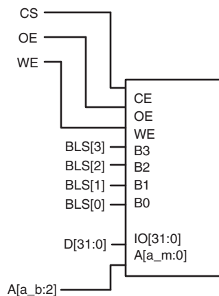
Fig 6. 32 bit bank external memory interfaces (BGFGx Bits MW = 10)
