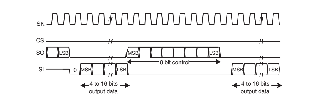
Fig 52. Microwire frame format (continuous transfers)
