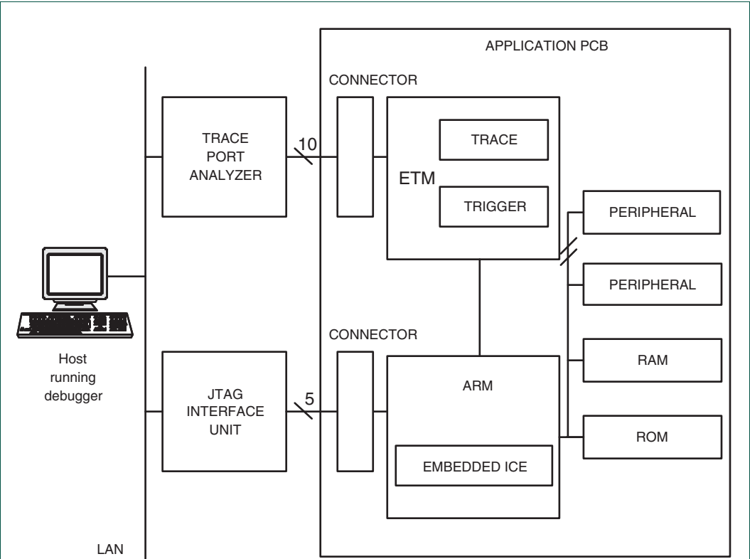
Fig 66. ETM debug environment block diagram
