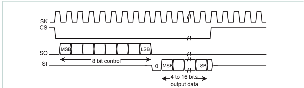
Fig 51. Microwire frame format (single transfer)
