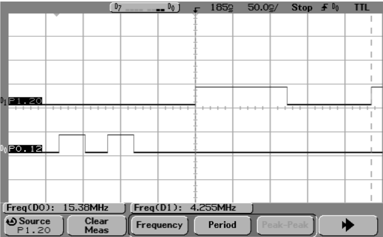
Fig 21. Illustration of the fast and slow GPIO access and output showing 3.5 x increase of the pin output frequency
