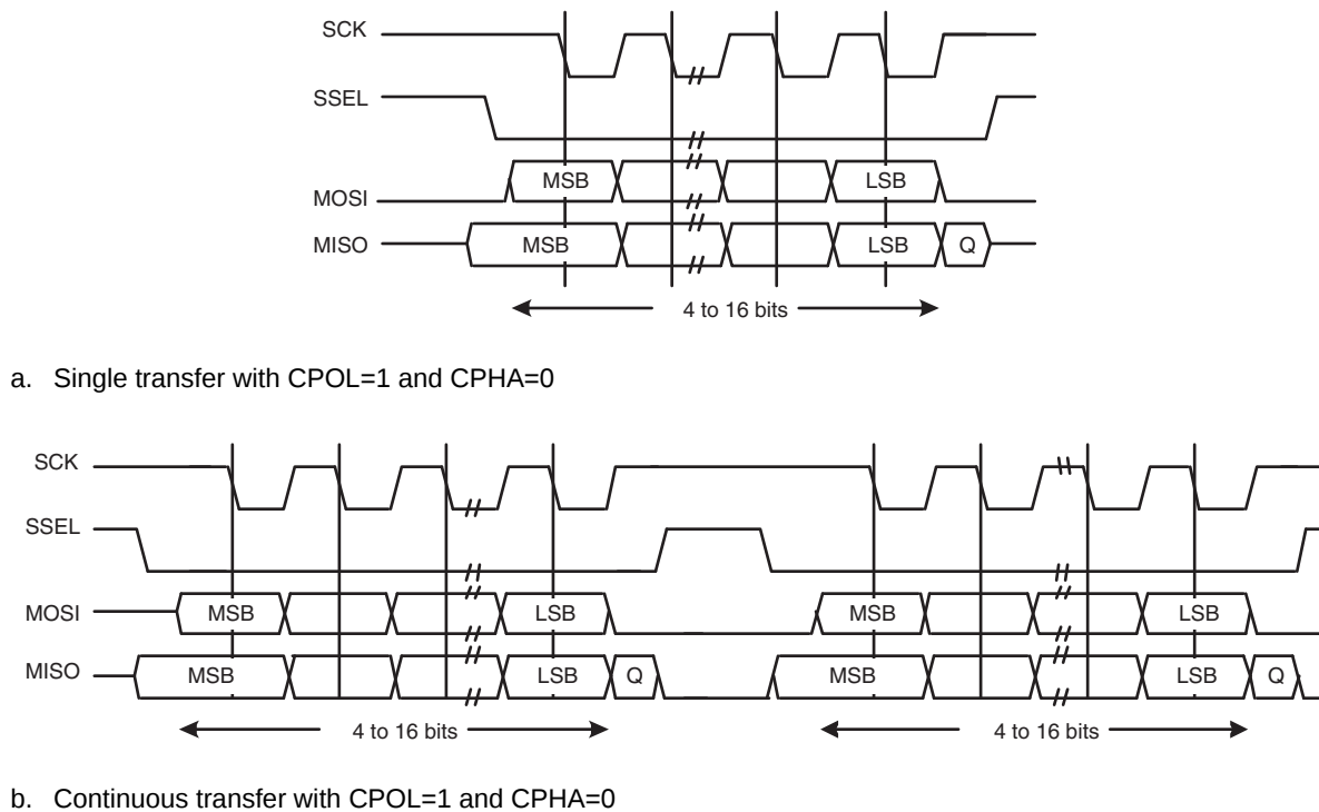
Fig 49. SPI frame format with CPOL = 1 and CPHA = 0 ( a) single and b) continuous transfer)
