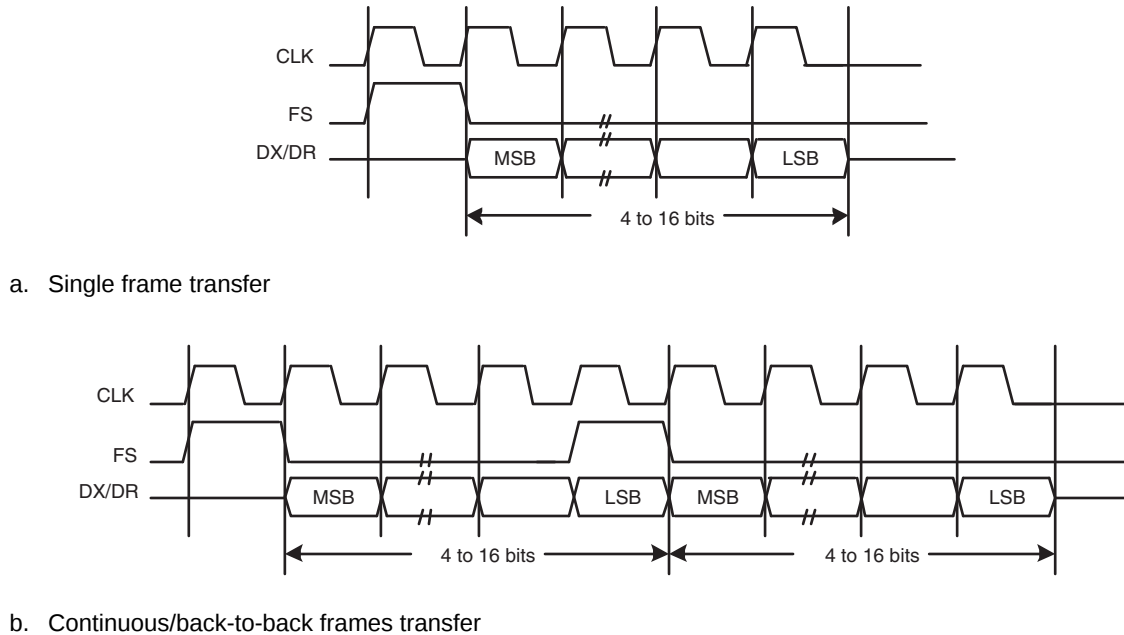
Fig 46. Texas Instruments synchronous serial frame format: a) single frame transfer and b) continuous/back-to-back two frames.
