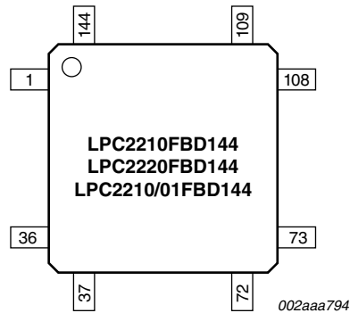
Fig 19. LPC2210/2220 and LPC2210/01 pin configuration for 144-pin LQFP package
