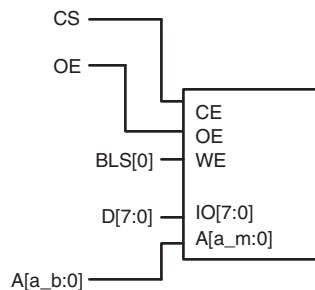
Fig 8. 8 bit bank external memory interface (BCFGx bits MW = 00 and RBLE = 0)
