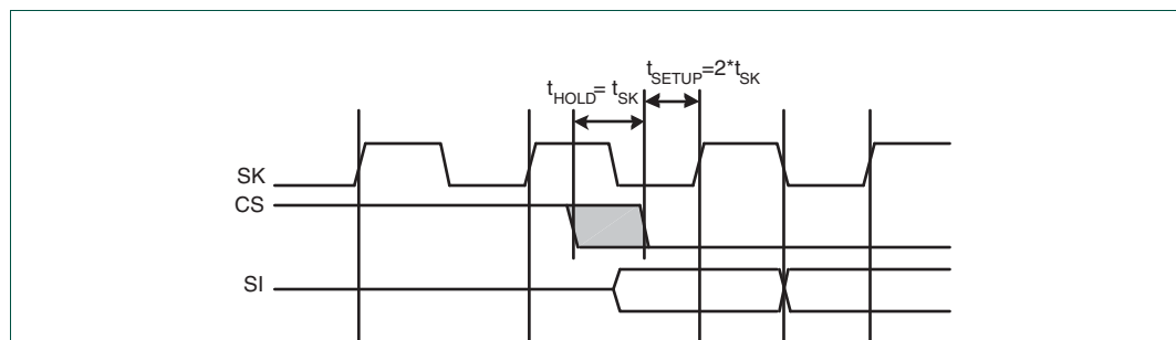
Fig 53. Microwire frame format (continuous transfers, details)
