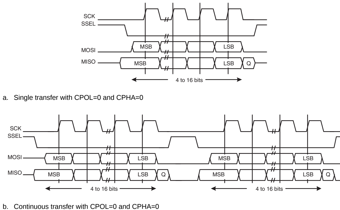
Fig 47. Motorola SPI frame format with CPOL=0 and CPHA=0 ( a) single transfer and b) continuous transfer)
