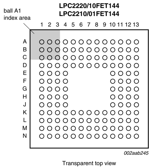
Fig 20. Ball configuration diagram for 144-pin TFBGA package
