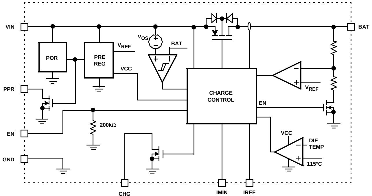
FIGURE 11. BLOCK DIAGRAM
