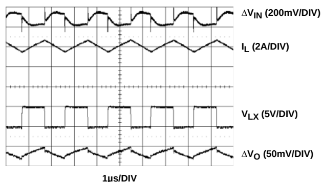
FIGURE 13. STEADY-STATE OPERATION
