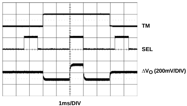
FIGURE 16. VOLTAGE MARGINING
