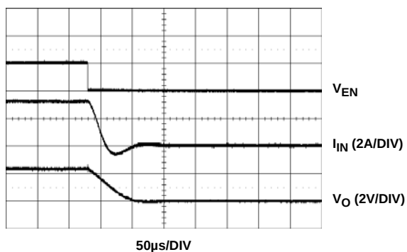
FIGURE 14. SHUT-DOWN
