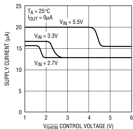
Supply Current vs V_{\overline{\text{SHDN}}}
