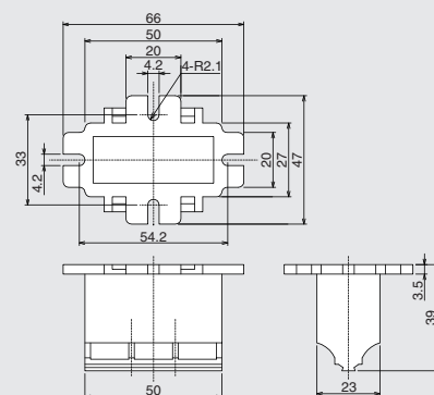
Auxiliary mounting bracket
