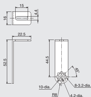
Mounting bracket
