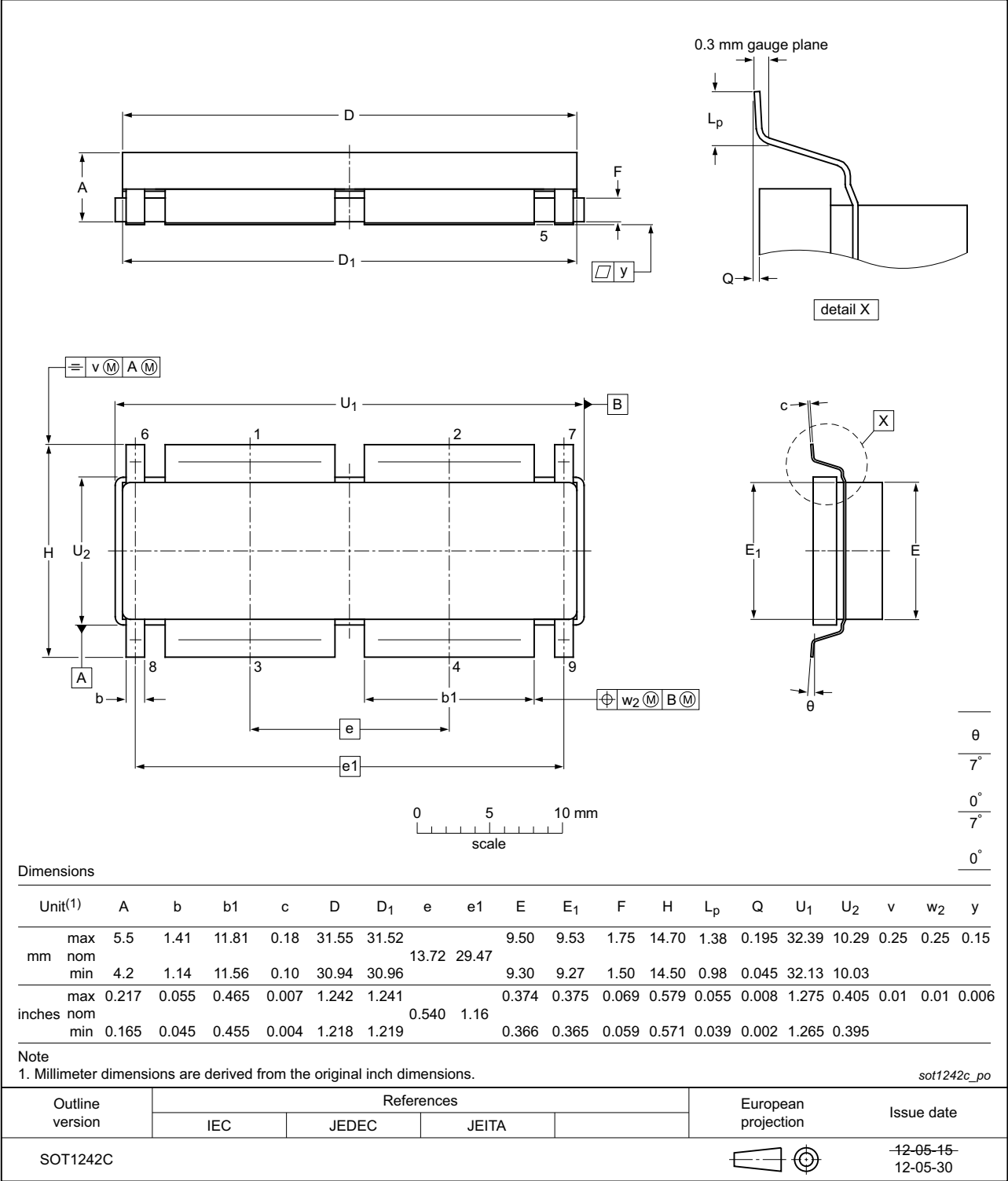
Earless flanged ceramic package; 8 leads SOT1242C
