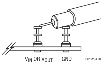
Figure 2. Measuring Input or Output Ripple
