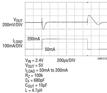
Load Transient 50mA to 200mA
