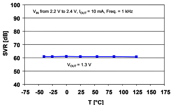
Figure 20. Supply voltage rejection vs. temperature ( V_{OUT} = 1.3\text{ V} )
