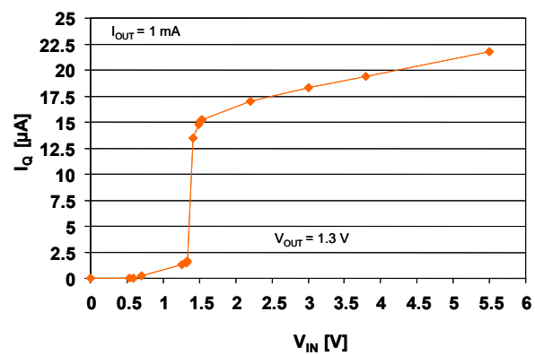
Figure 17. Quiescent current vs. input voltage
