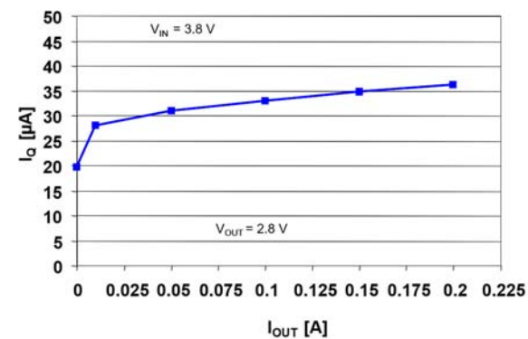
Figure 18. Quiescent current vs. output current
