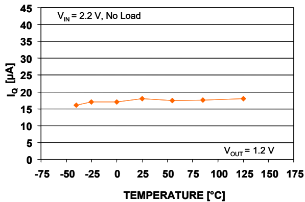
Figure 14. Quiescent current vs. temperature ( V_{OUT} = 1.2\text{ V} , I_{OUT} = 0\text{ mA} )
