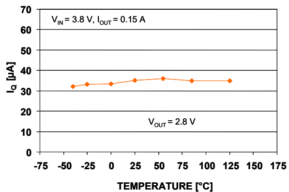
Figure 16. Quiescent current vs. temperature ( V_{OUT} = 2.8\text{ V} , I_{OUT} = 0.15\text{ A} )
