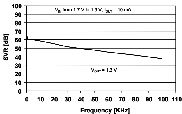
Figure 25. Supply voltage rejection vs. frequency ( V_{OUT} = 1.3\text{ V} )
