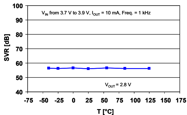
Figure 21. Supply voltage rejection vs. temperature (Freq. = 1 kHz)
