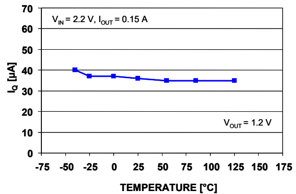
Figure 15. Quiescent current vs. temperature ( V_{OUT} = 1.2\text{ V} , I_{OUT} = 0.15\text{ A} )
