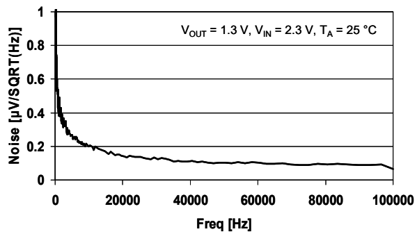
Figure 28. LD39115J noise
