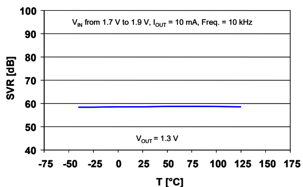
Figure 22. Supply voltage rejection vs. temperature (Freq. = 10 kHz)
