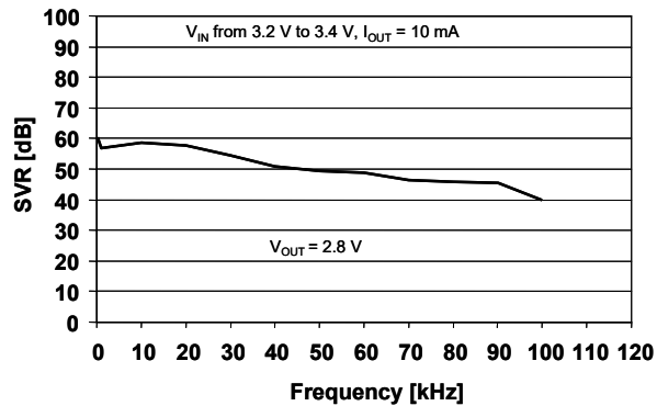
Figure 26. Supply voltage rejection vs. frequency ( V_{OUT} = 2.8 \text{ V} )
