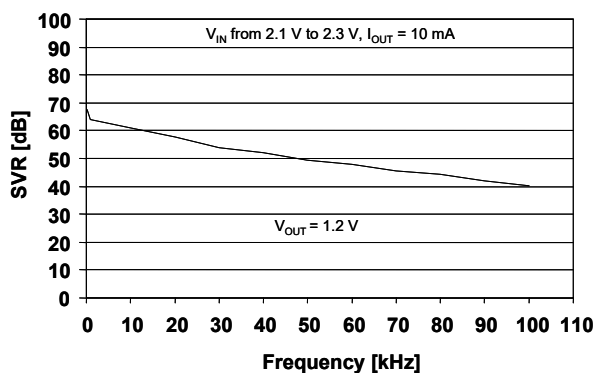
Figure 24. Supply voltage rejection vs. frequency ( V_{OUT} = 1.2\text{ V} )
