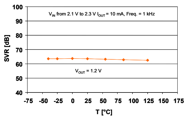
Figure 19. Supply voltage rejection vs. temperature ( V_{OUT} = 1.2\text{ V} )
