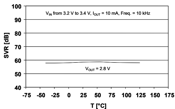
Figure 23. Supply voltage rejection vs. temperature ( V_{OUT} = 2.8\text{ V} )
