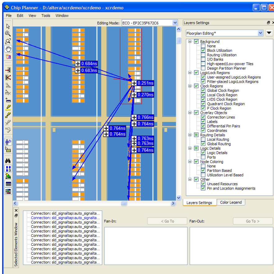
Figure 5. Chip Planner
