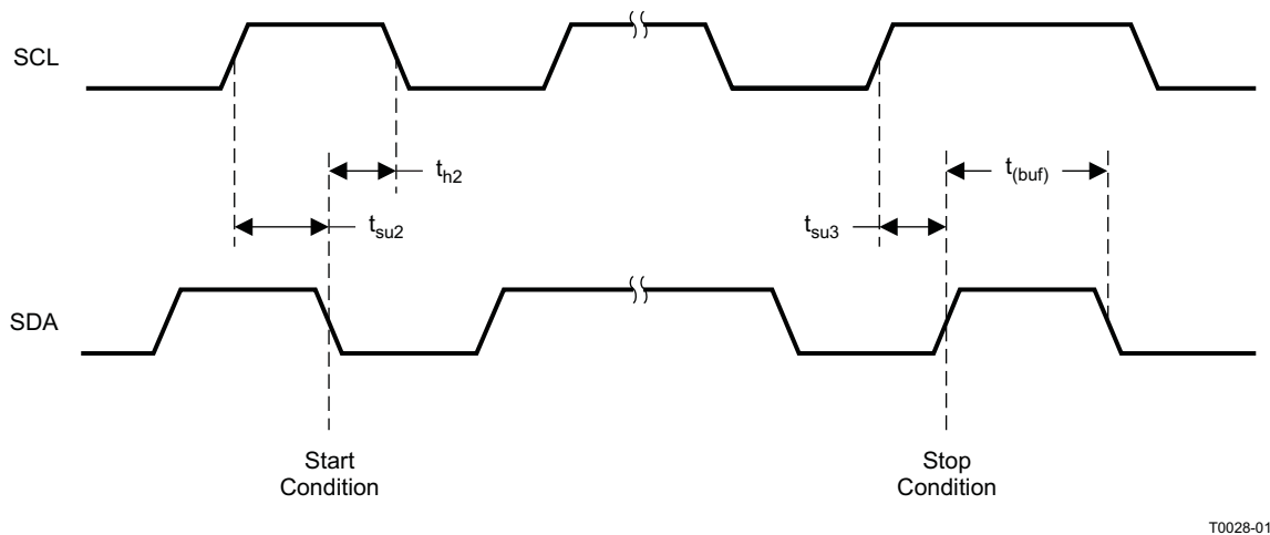
Figure 2. Start and Stop Conditions Timing
