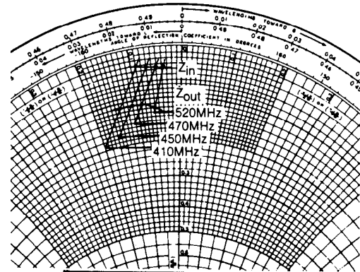
SERIES INPUT AND OUTPUT IMPEDANCE VS. FREQUENCY
