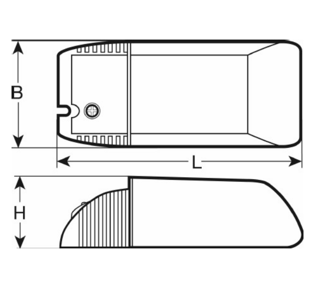
Product line drawing OTe 9/220...240/700 PC | OTe 9/220...240/350 PC | OTe 15/220...240/700 PC | OTe 15/220...240/350 PC | OTe 20/220...240/350 PC | OTe 20/220...240/700 PC
