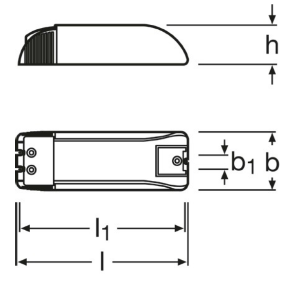
Product line drawing OTe 35/220...240/700 PC
