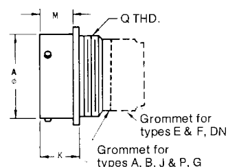
Crimp KPSE01/MS3121
