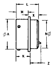
Solder KPT02/MS3112
