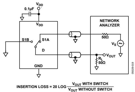
Figure 26. Bandwidth
