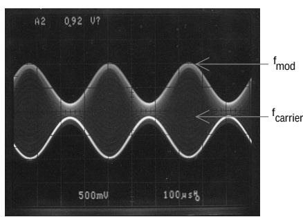
FIGURE 9. Output signal per the Circuit of Figure 8
