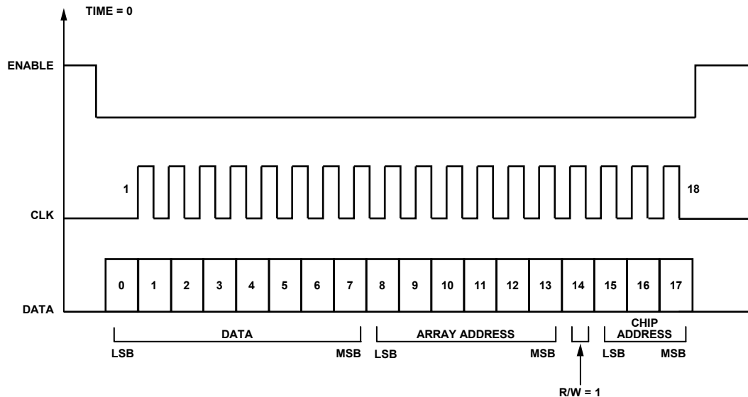
Figure 17. Timing Diagram for Writing a Row of the Receiver Serial Interface
