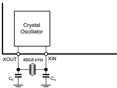
Figure 12. Crystal Oscillator
