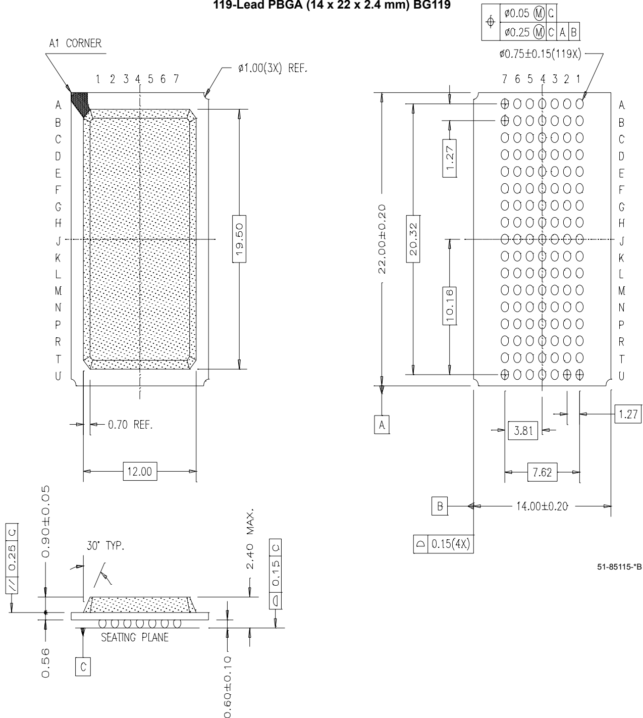
119-Lead PBGA (14 x 22 x 2.4 mm) BG119
