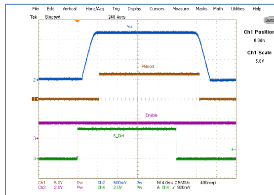
Figure 44: Start/Stop using S-ctrl pin Ch1-PGood,Ch2:Vout;Ch3-EN.Ch4-S-Ctrl
