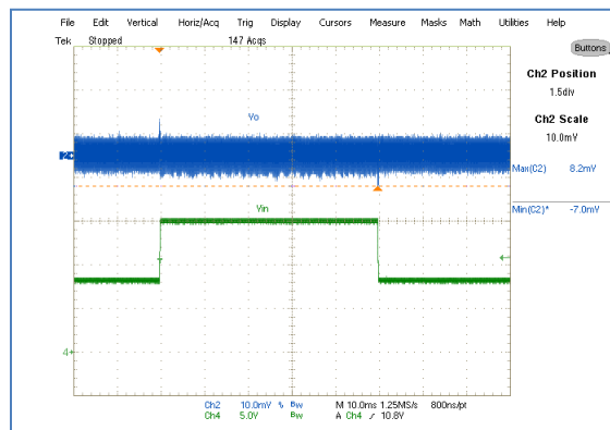
Figure 43: Feed Forward for V_{in} change from 7-16-VV Ch2:Vo,Ch4:Vin
