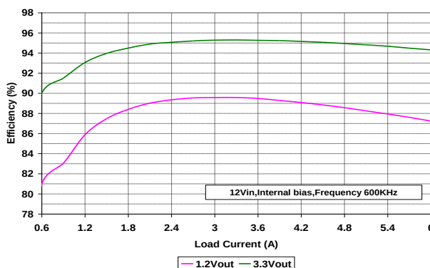
Figure 2: IR3898 Efficiency
