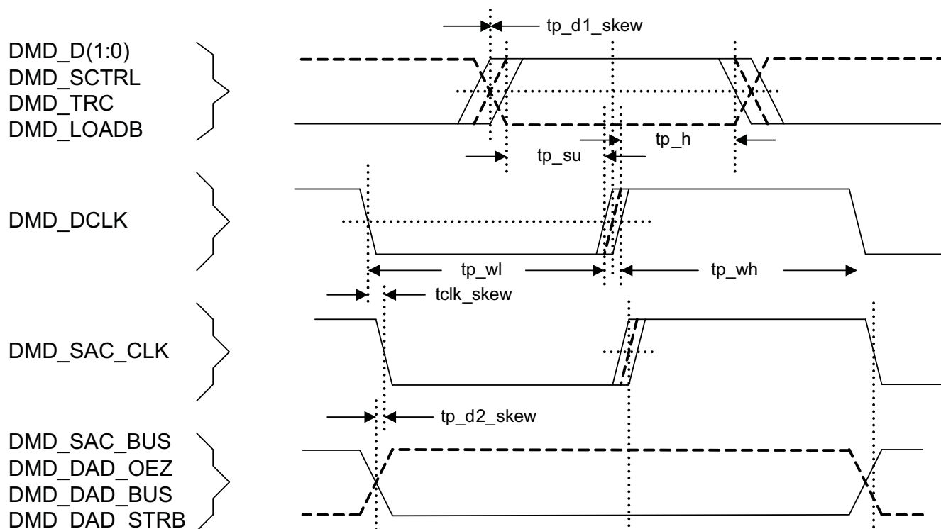
Figure 10. DMD I/F Timing
